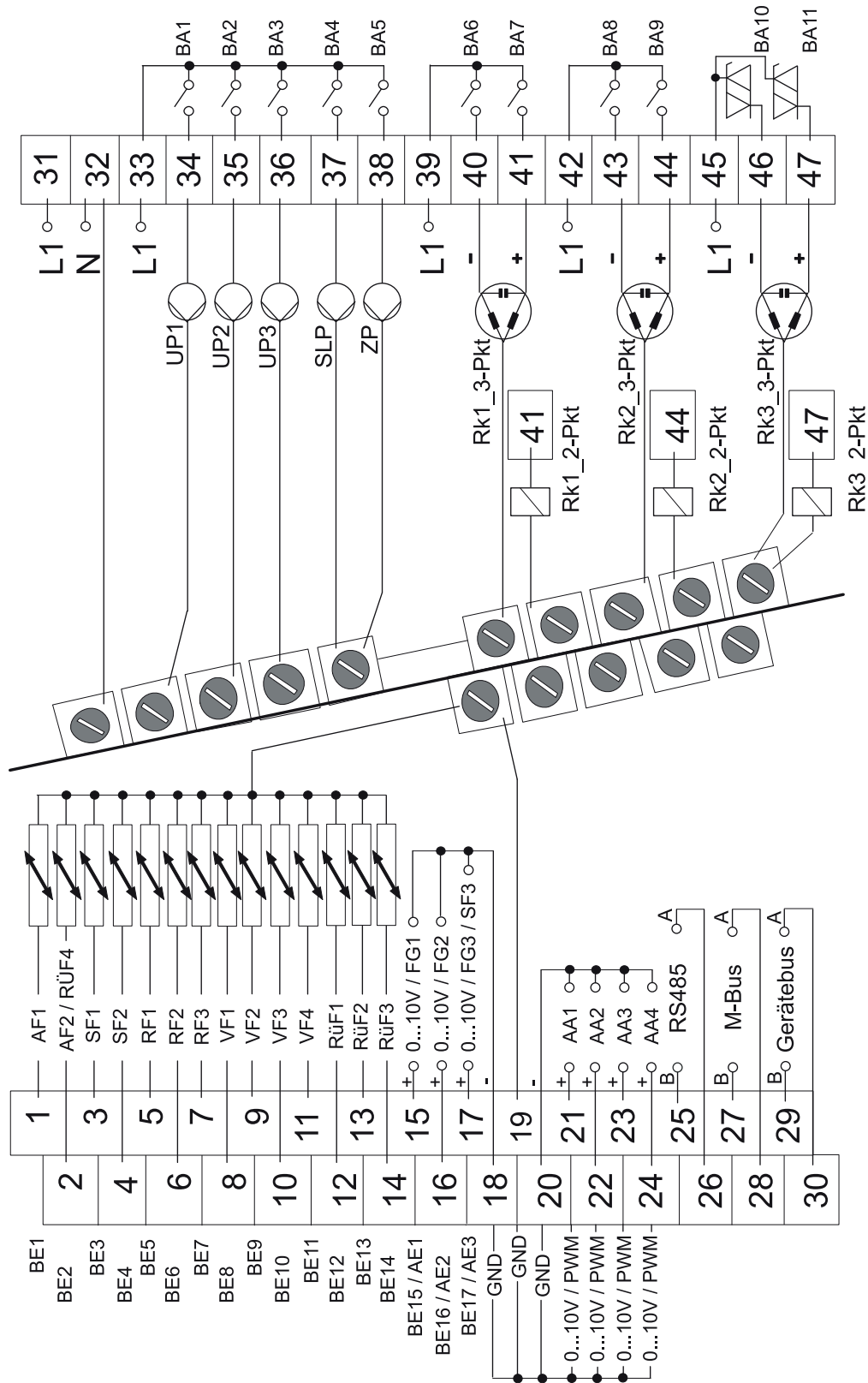
Fig. 5: Electrical connection of the TROVIS 5578-1114 Heating Controller
