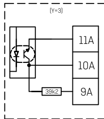
Figure 14. Block diagram for galvanically separated output module (Y=3).
