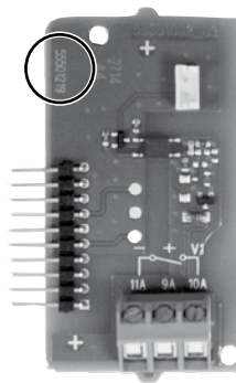
Figure 15. Galvanically separated output module (Y=3). Note the PCB number 5550-1219 in the encircled area.
